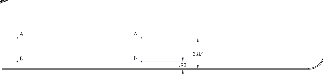
Figure 1 Recommended Pre-Drill on Rectangular Tables Only Note: not all tables support above pre-drill locations
