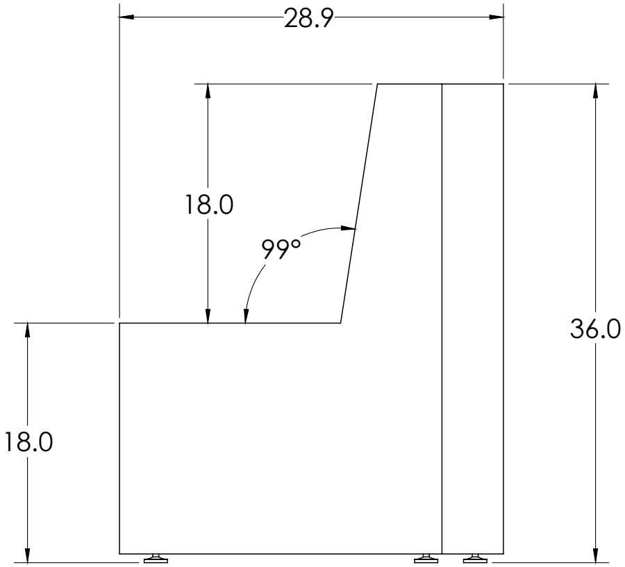
SIDE VIEW
