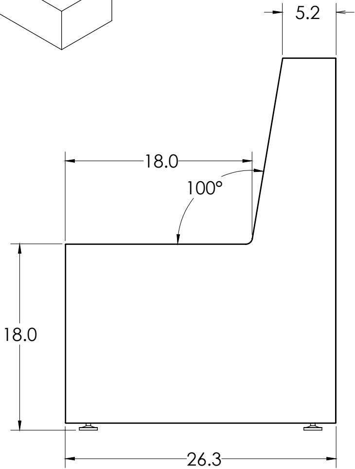
SIDE VIEW
